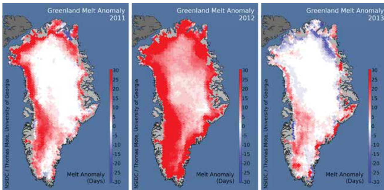
Greenland melt anomalies
