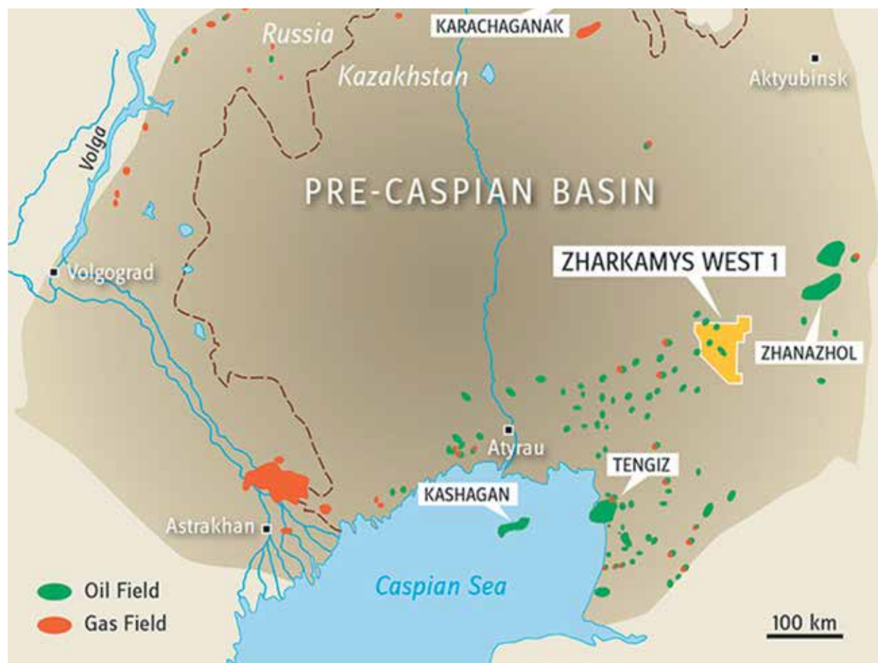
Figure 3. The Pre-Caspian basin
