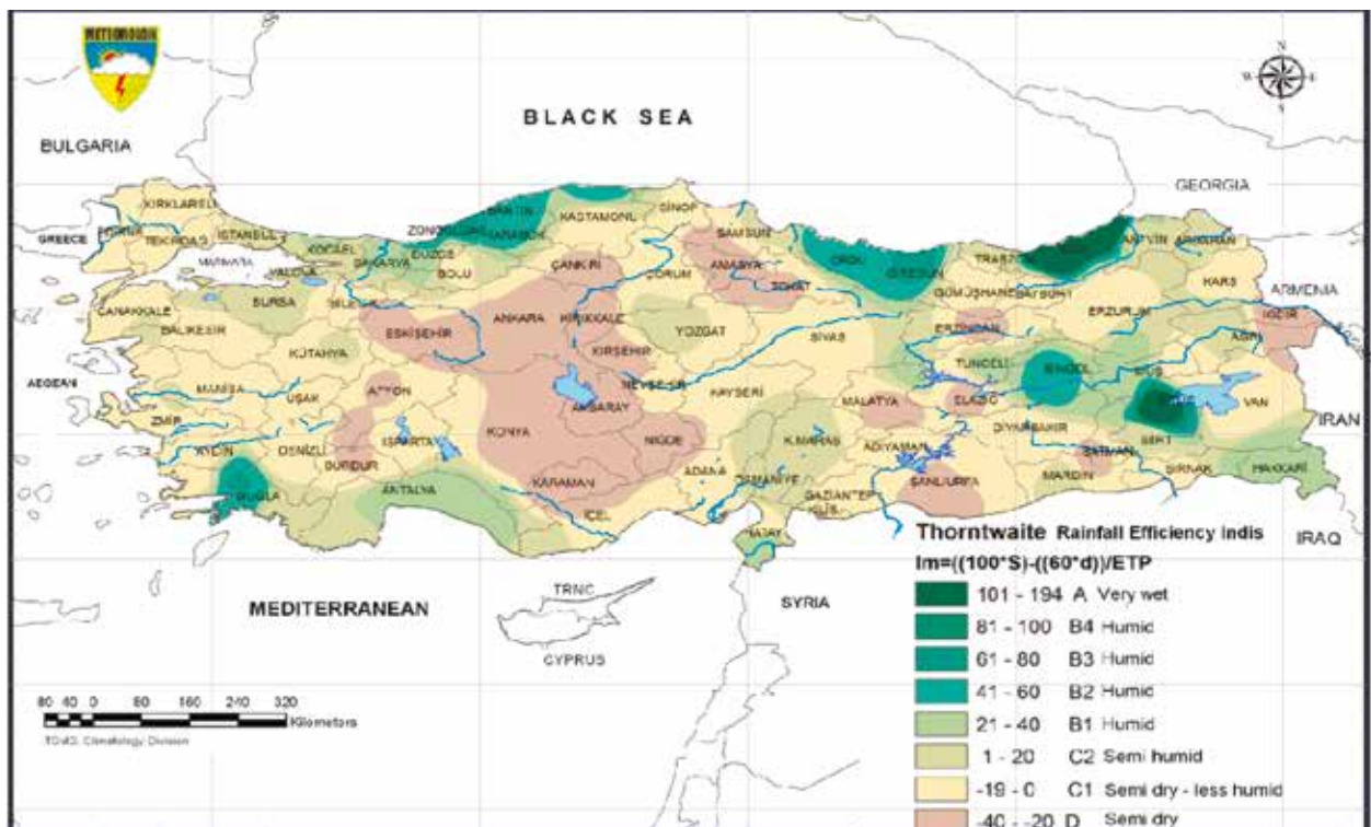
Figure 2. Turkey’s climate according to the Thornthwaite climate classification (Source: Sensoy et al., 2016).
