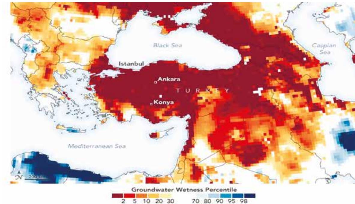
Figure 3. Map of the shallow groundwater storage in aquifers measured using Gravity Recovery and Climate Experiment Follow On (GRACE-FO) satellites (Source: Dauphin, L., NASA Earth Observatory).
